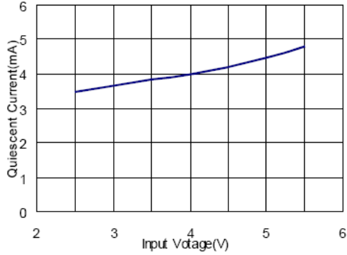
11. Quiescent Current
