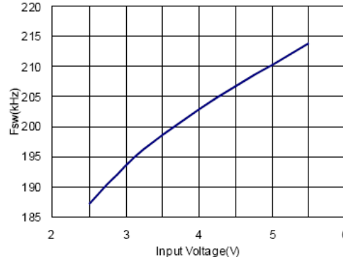
12. Switching Frequency
