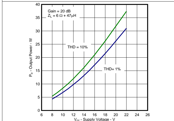
Figure 17. Output Power vs Supply Voltage (BTL)
