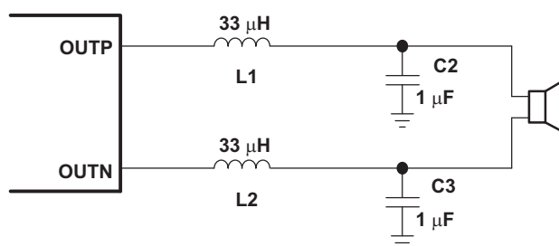
Figure 38. Typical LC Output Filter, Cutoff Frequency of 27 KHz, Speaker Impedance = 8 Ω
