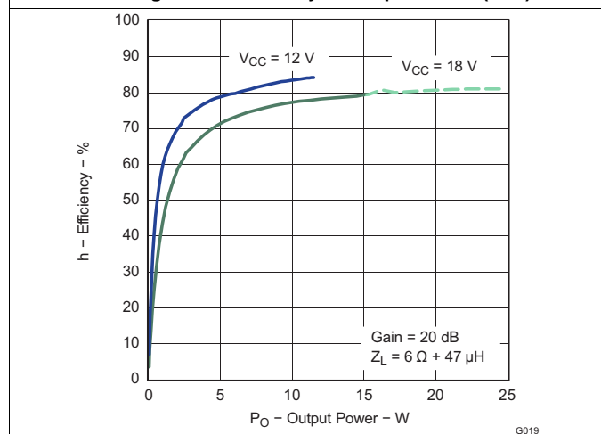
Note: Dashed Lines represent thermally limited regions. Figure 21. Efficiency vs Output Power (BTL)
