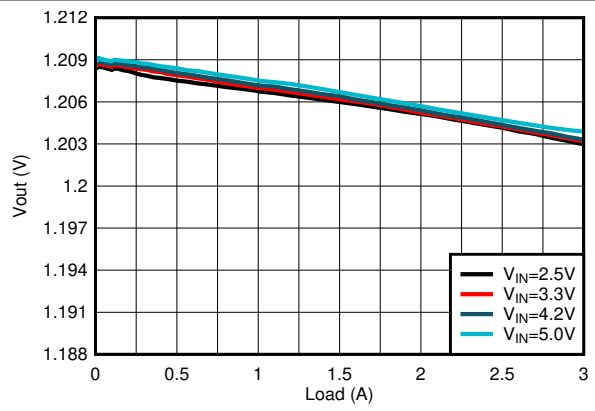
Figure 9-14. Load Regulation
