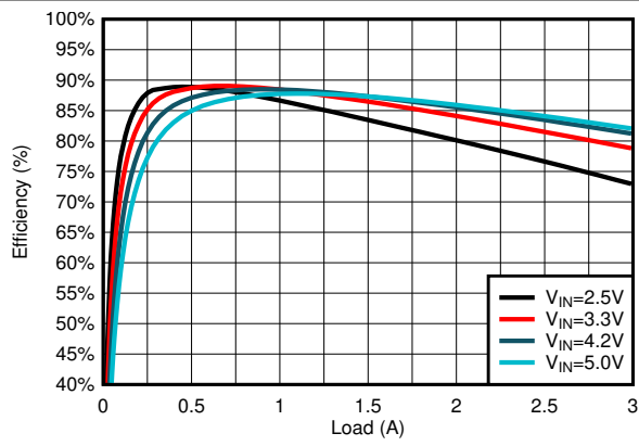
Figure 9-11. Efficiency
