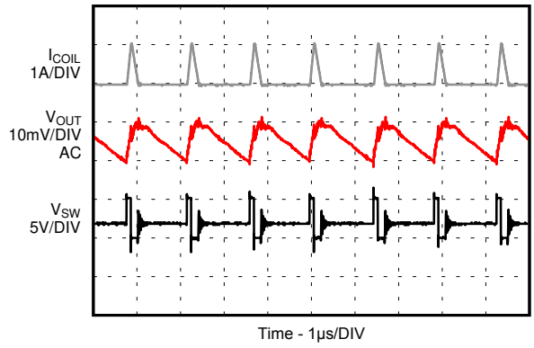
Figure 9-28. PSM Operation
