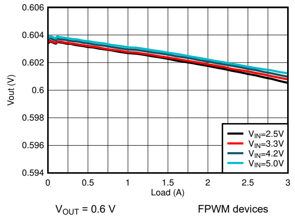
Figure 9-6. Load Regulation
