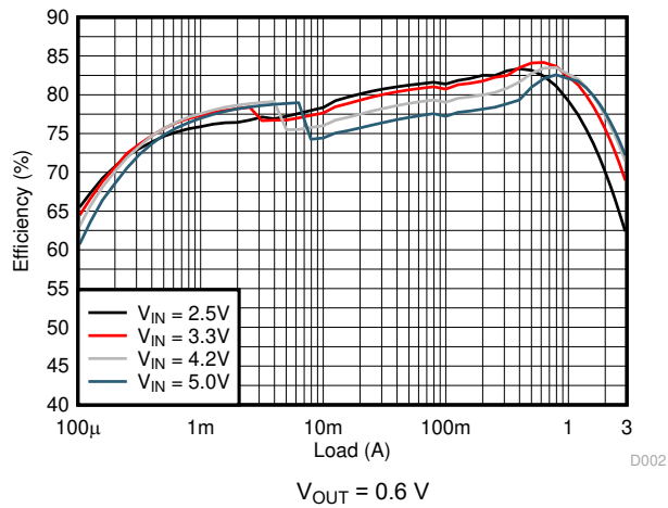
Figure 9-3. Efficiency
