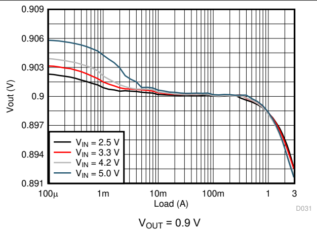
Figure 9-8. Load Regulation
