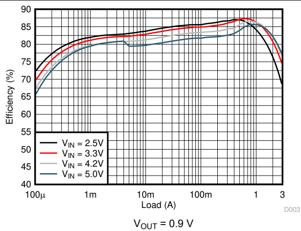
Figure 9-7. Efficiency
