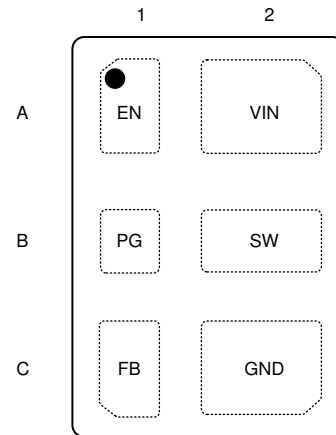
Figure 6-2. YWC Package Top View
