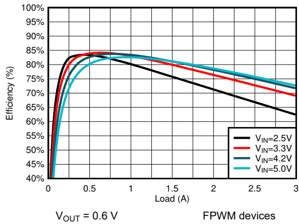
Figure 9-5. Efficiency
