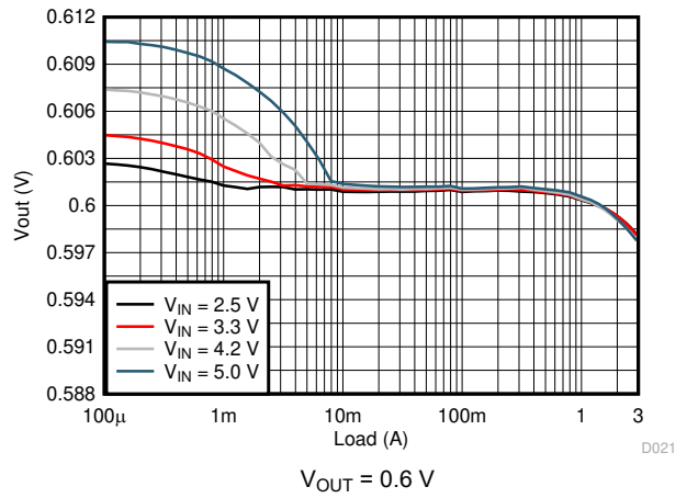
Figure 9-4. Load Regulation
