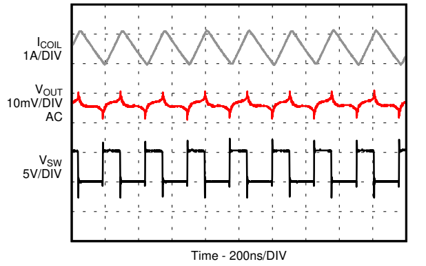
Figure 9-27. PWM Operation
