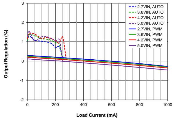
Figure 11. \Delta V_{OUT} (%) vs. Load Current and Input Voltage, V_{OUT} = 1.23\text{ V} , Normalized to 3.6\text{ V}_{IN} , 500 mA Load, FPWM, Dotted for Auto Mode
