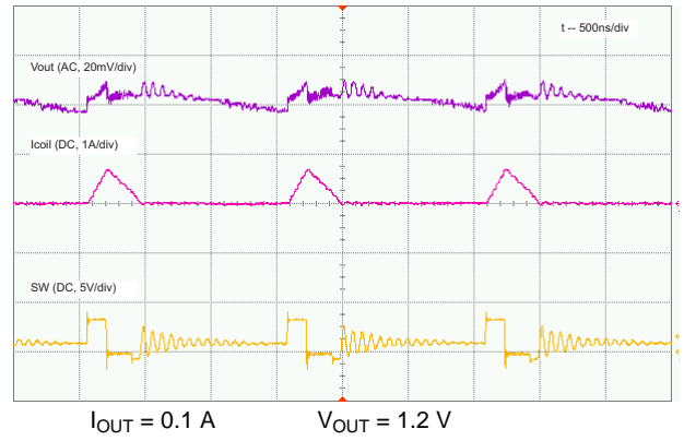
Figure 12. PFM Operation
