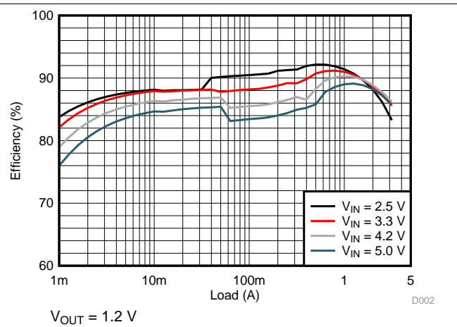
Figure 6. Efficiency
