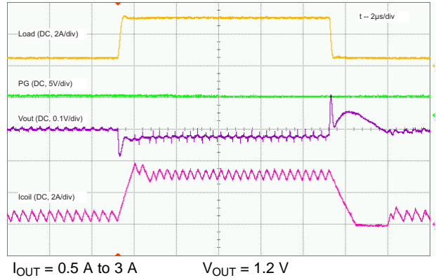
Figure 18. Load Transient
