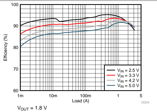
Figure 8. Efficiency
