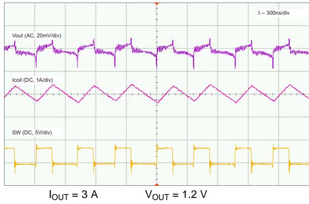
Figure 11. PWM Operation
