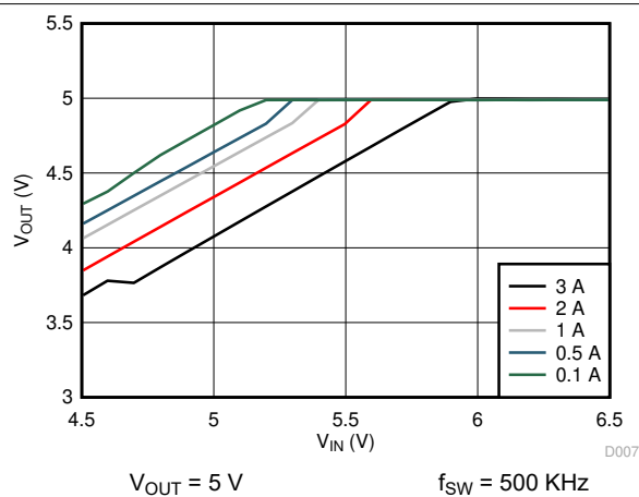
Figure 6-8. Dropout Curve
