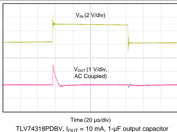
Figure 23. Line Transient
