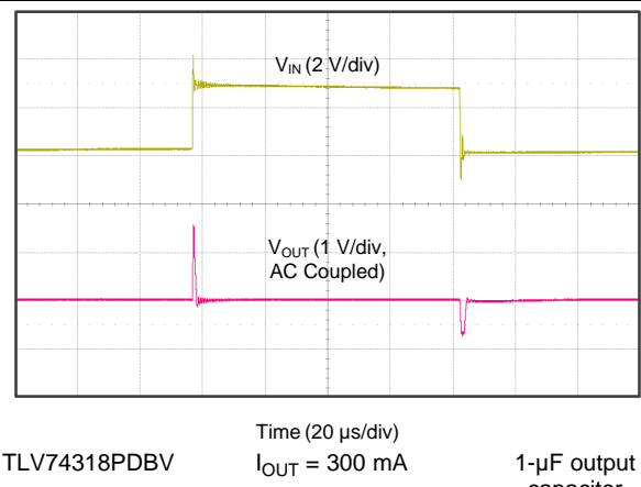
Figure 24. Line Transient
