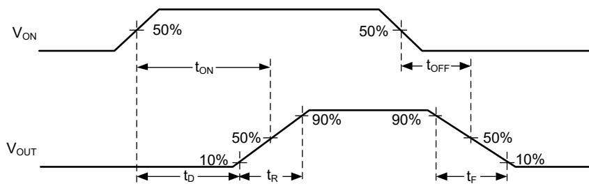
Figure 3. Timing Waveforms
