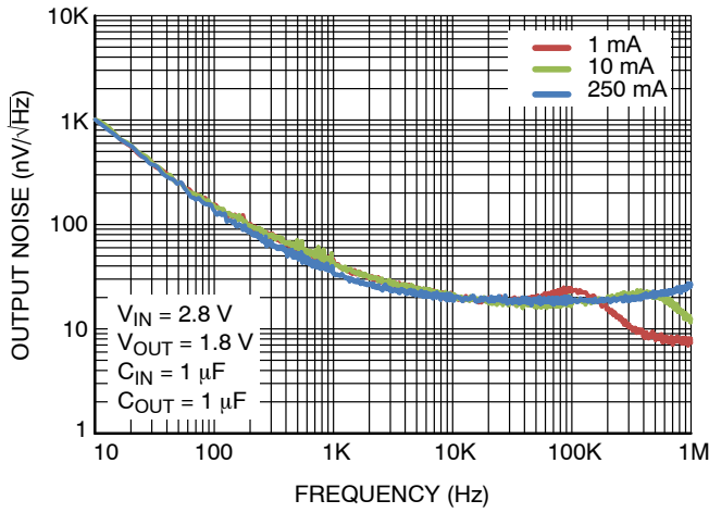
Figure 27. Output Voltage Noise Spectral Density – V_{OUT} = 1.8 V
