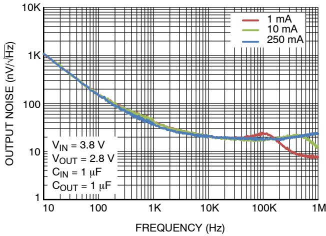
Figure 28. Output Voltage Noise Spectral Density – V_{OUT} = 2.8 V
