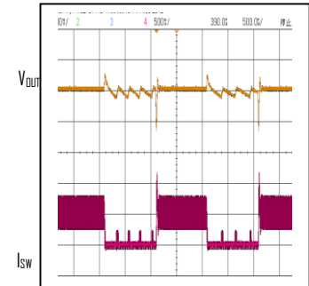
Load Transient Response V_{IN}=12\text{V}, V_{OUT}=3.3\text{V}, I_{OUT}=0\text{ to }0.5\text{A}
