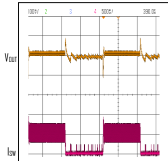
Load Transient Response V_{IN}=12\text{V}, V_{OUT}=5\text{V}, I_{OUT}=0\text{ to }0.5\text{A}
