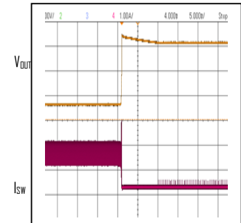
Short-Circuit Recovery V_{IN}=24\text{V}, V_{OUT}=5\text{V}, I_{OUT}=Short\text{ to }0\text{A}
