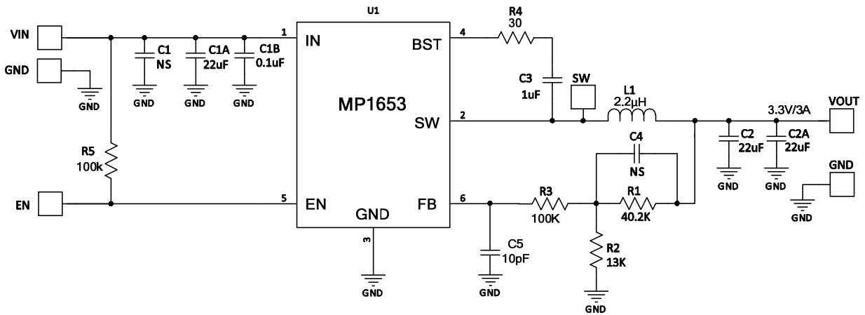
Figure 6: V_{IN}=12V , V_{OUT}=3.3V/3A
