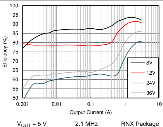
Figure 9-17. Efficiency
