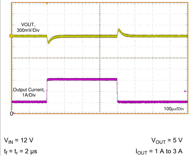
Figure 9-24. Load Transient
