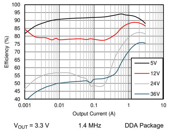
Figure 9-10. Efficiency
