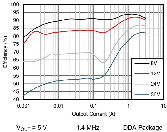
Figure 9-9. Efficiency
