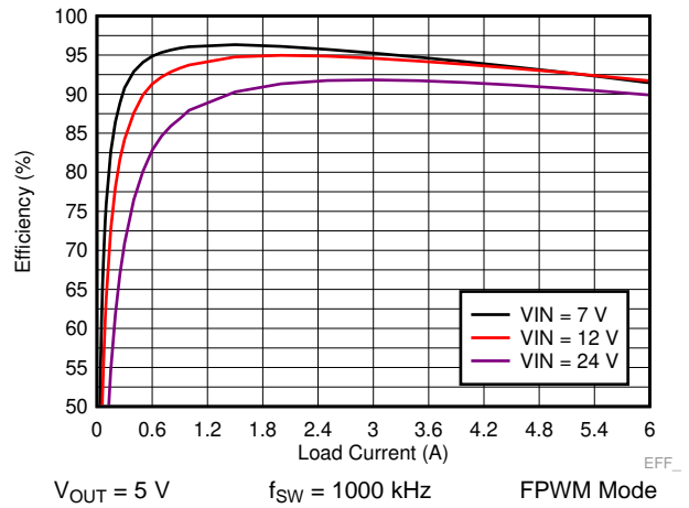
Figure 36. LM73606 Efficiency
