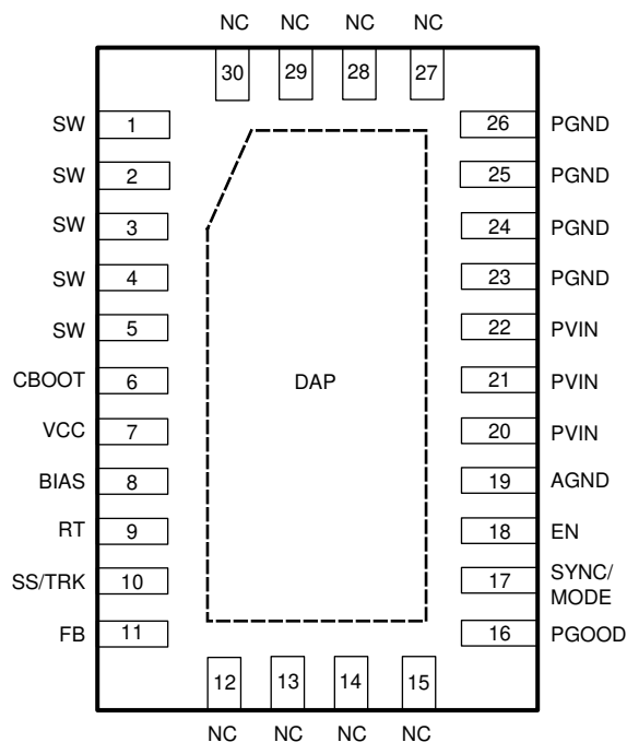
Pin Functions
