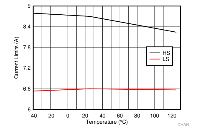
Figure 5. LM73605 High-Side and Low-Side Current Limit
