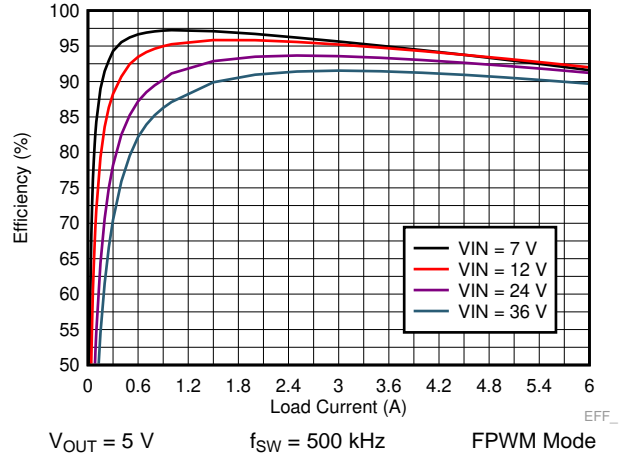
Figure 34. LM73606 Efficiency
