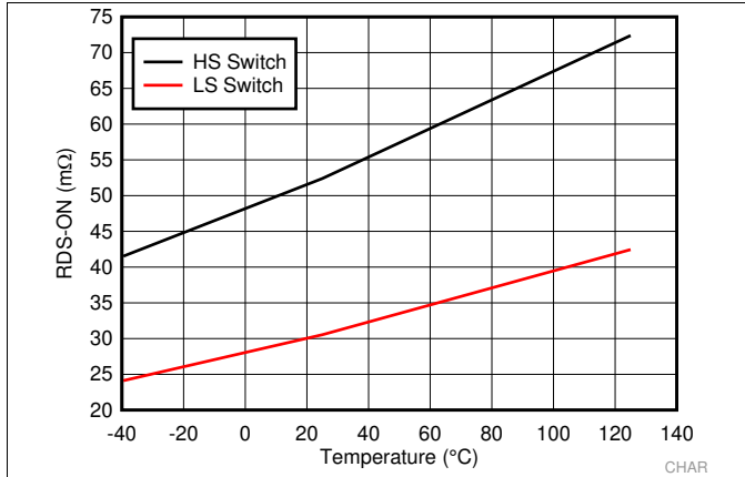
Figure 1. High-Side and Low-Side Switches R_{DS-ON}
