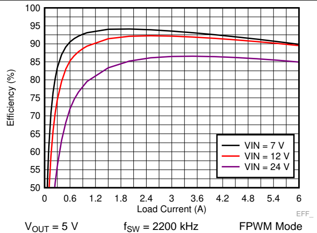
Figure 38. LM73606 Efficiency
