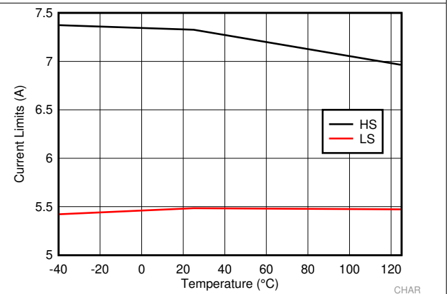
Figure 4. LM73605 High-Side and Low-Side Current Limits
