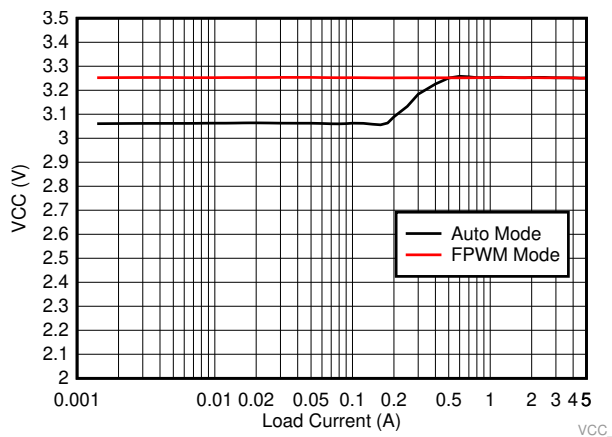
Figure 17. VCC Voltage versus Load Current
