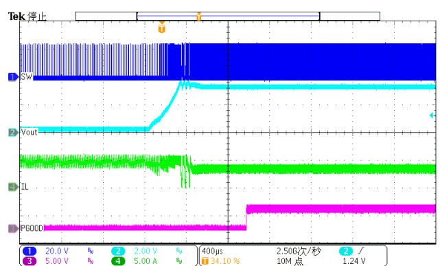
Figure 17. Over Current Release (hard short to 3A)
