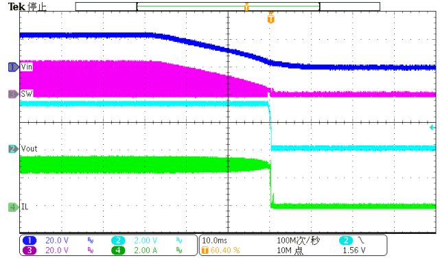
Figure 13. Power down(Iload=3A)
