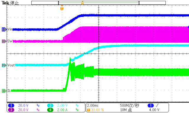
Figure 12. Power up(Iload=3A)
