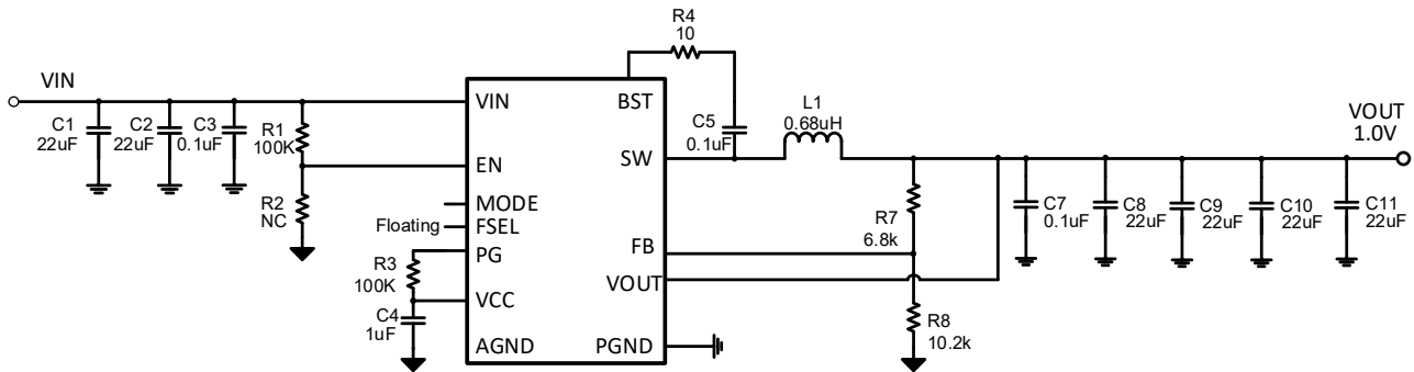
Figure 16. SCT2260A Design Example, 1V Output
