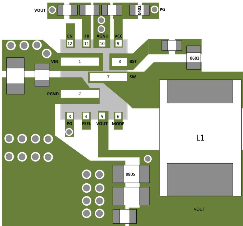
Figure 26. PCB Layout Example
