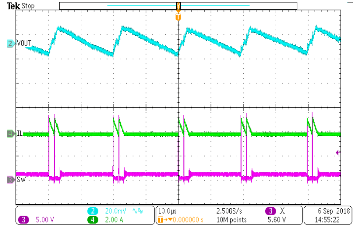
Figure 18. Switching Waveforms and Output Ripple in USM (IOUT=100mA)
