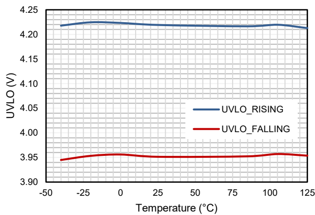
Figure 6. VIN VULO vs Temperature
