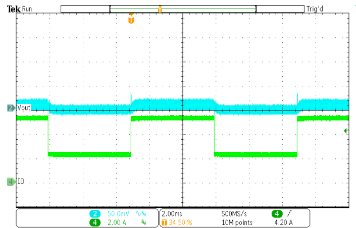
Figure 22. Load Transient (Vout=1V, Iout=3A to 6A)
