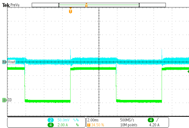
Figure 21. Load Transient (Vout=1V, Iout=0.6A to 5.4A)
