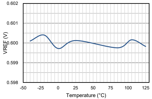
Figure 9. Reference Voltage vs Temperature
