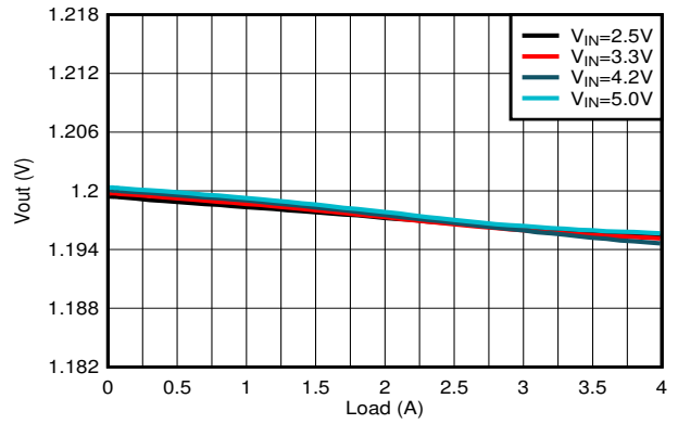
Figure 9-10. Load Regulation
