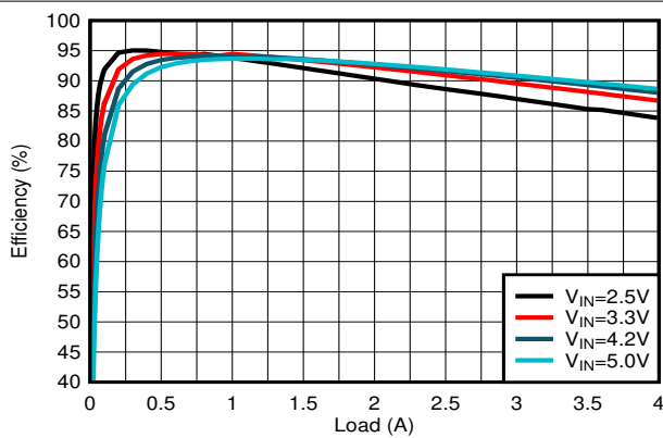
Figure 9-11. Efficiency
