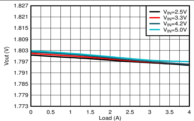
Figure 9-12. Load Regulation
