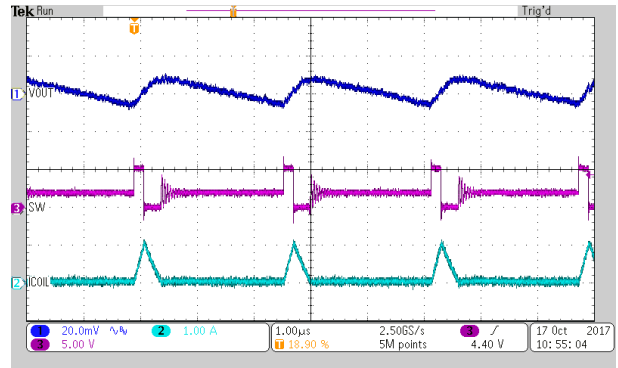
Figure 9-34. PSM Operation
