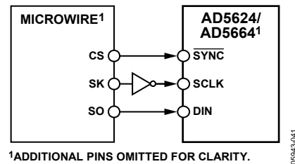
Figure 39. MICROWIRE Interface to AD5624/AD5664
