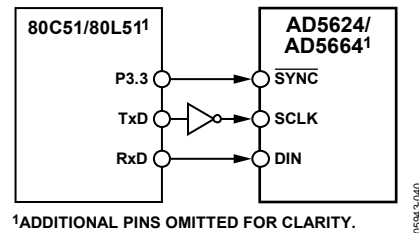
Figure 38. 80C51/80L51 Interface to AD5624/AD5664
