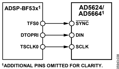
Figure 36. Blackfin ADSP-BF53x Interface to AD5624/AD5664
