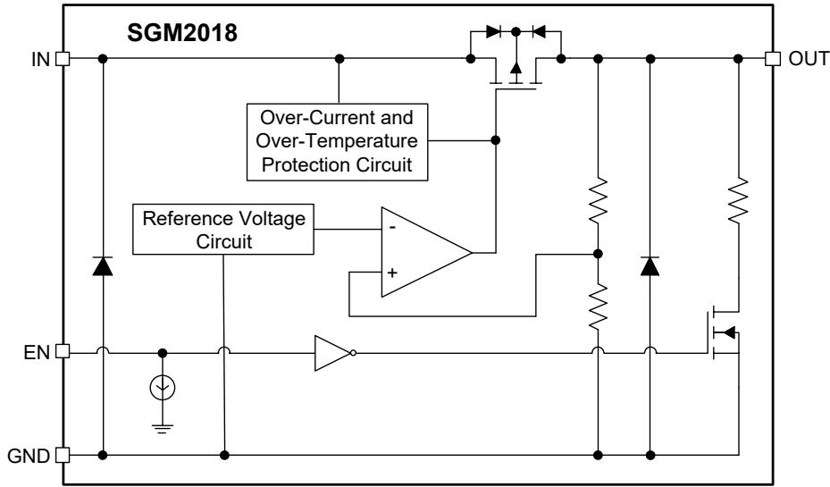
Figure 1. Block Diagram
