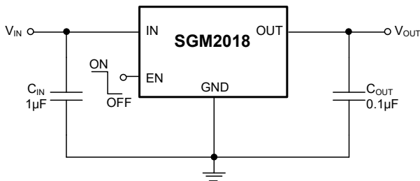
Figure 2. Application Circuit
