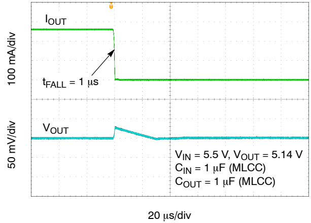
Figure 49. Load Transient Response – 250 mA to 1 mA – V_{OUT} = 5.14 V
