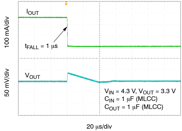
Figure 47. Load Transient Response – 250 mA to 1 mA – V_{OUT} = 3.3 V
