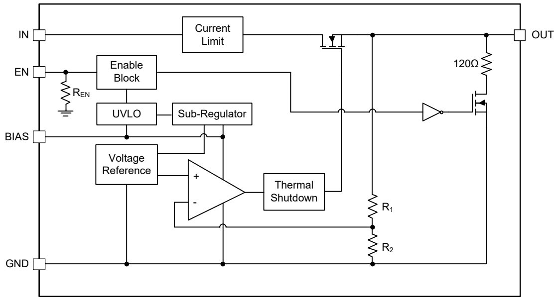
Figure 2. Block Diagram
