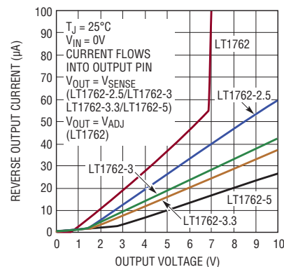
Figure 7. Reverse Output Current
