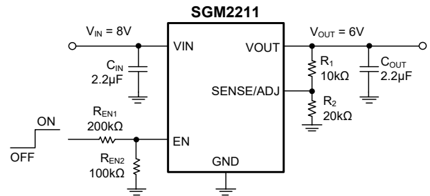
Figure 9. Typical EN Pin Voltage Divider
