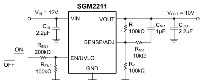
Figure 10. Noise Reduction Modification
