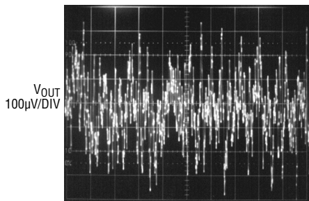
LT1763-5 10Hz to 100kHz Output Noise C BYP = 0
