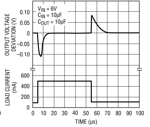
LT1763-5 Transient Response C_{BYP} = 0.01\mu\text{F}
