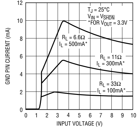
LT1763-3.3 GND Pin Current
