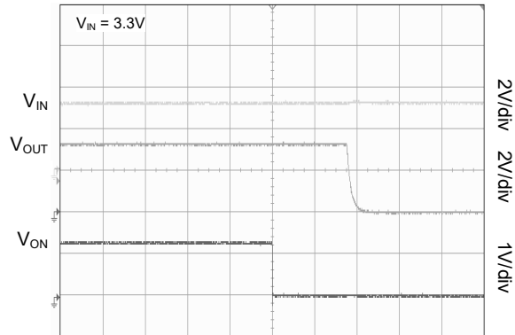
Time (10μs/div)
