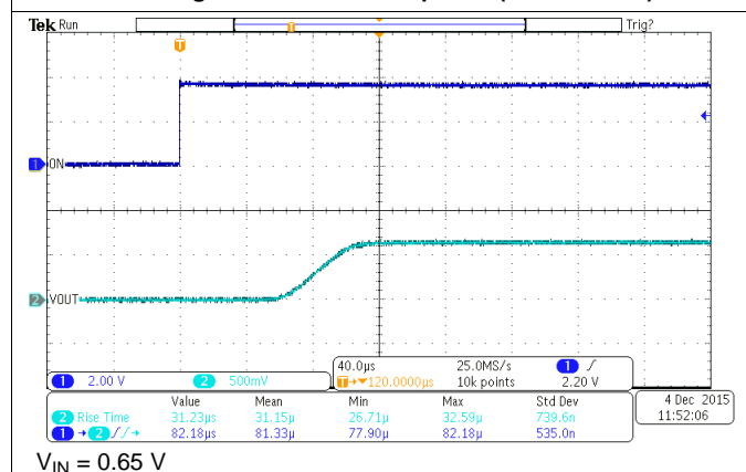
Figure 23. Turnon Response (TPS22925Cx)
