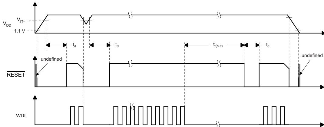
Figure 1. Timing Diagram
