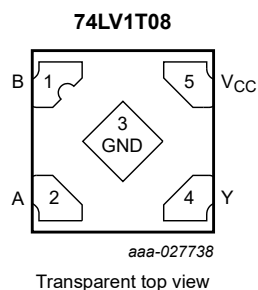
Fig. 5. Pin configuration SOT1226-3 (X2SON5)
