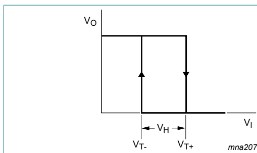
Fig. 8. Transfer characteristic
