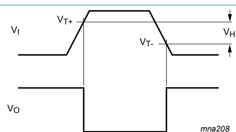
Fig. 9. Definition of V_{T+} , V_{T-} and V_H
