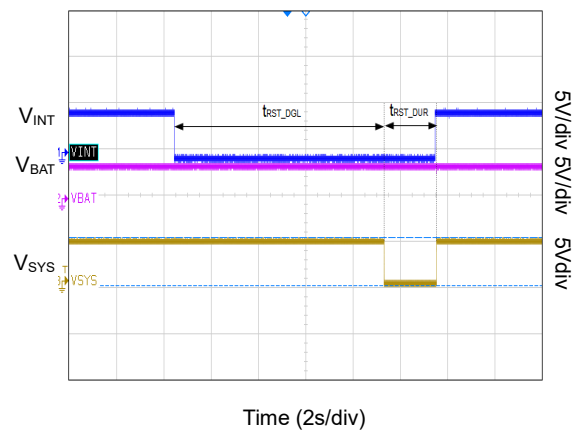
Figure 7. Power Recycling Waveforms
