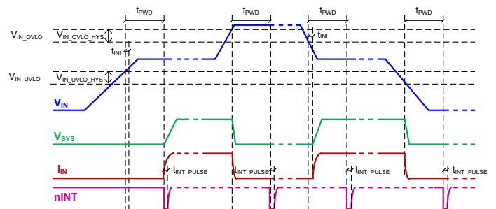
Figure 4. Input Power Detection and nINT Signaling Timings
