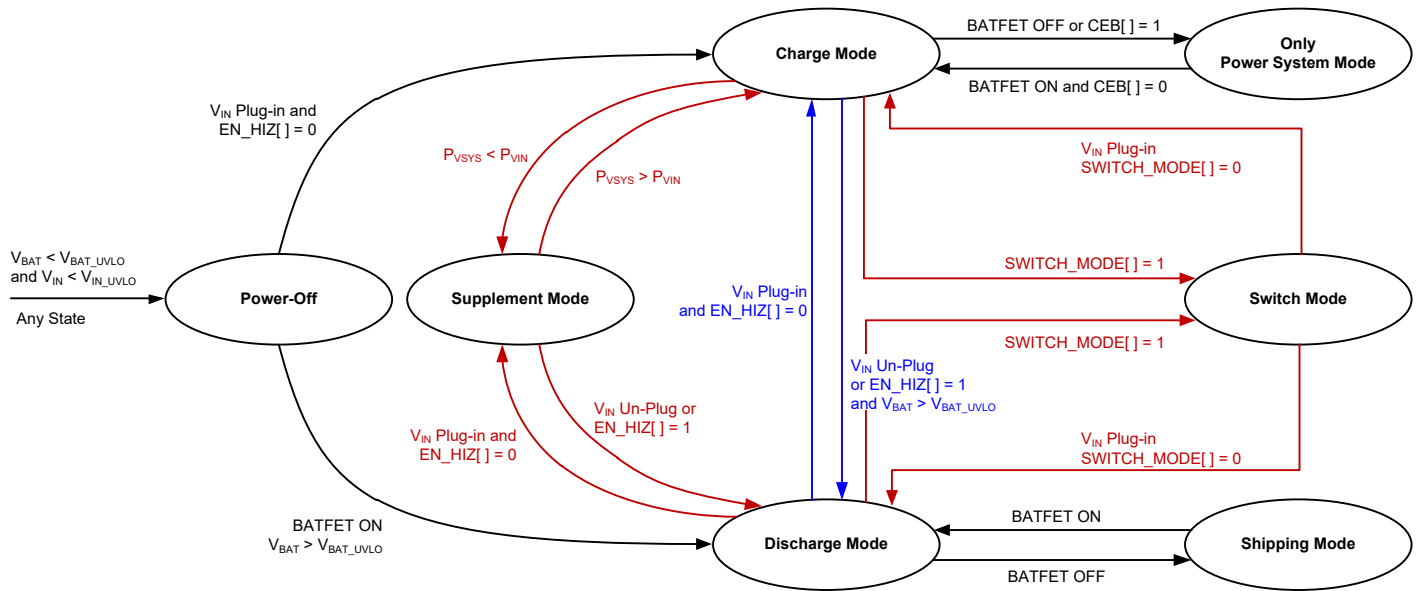
Figure 8. State Machine Conversion
