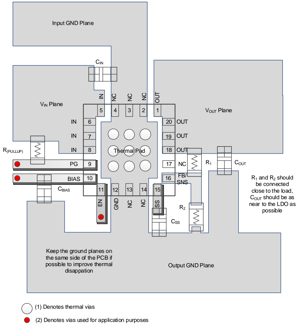
Figure 37. Layout Example (RGW Package)
