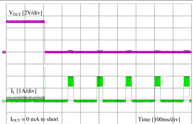
Figure 9-8. Short Protection
