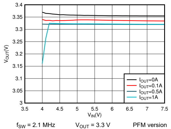
Figure 7-6. 3.3-V Dropout
