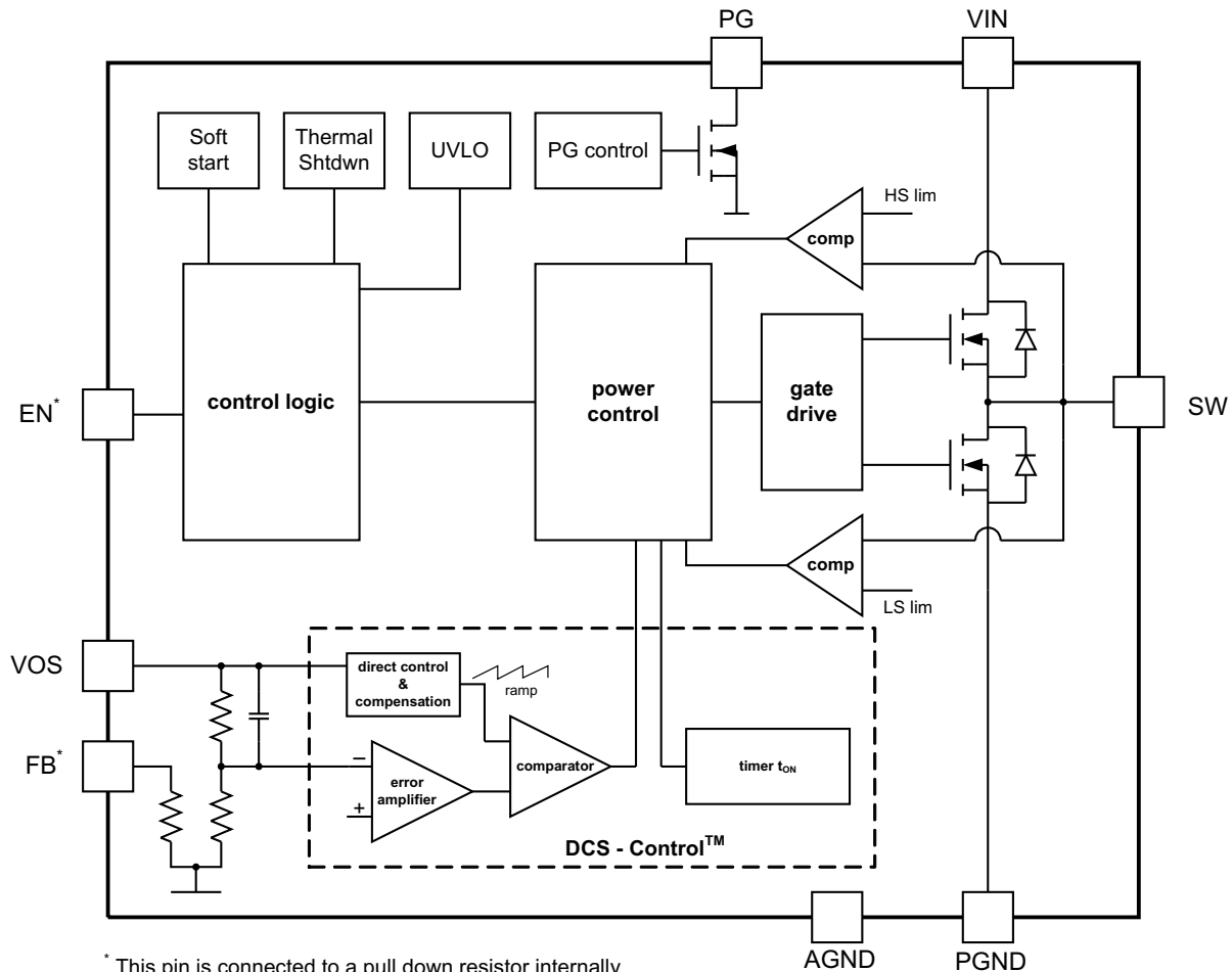
Figure 6. TPS62162-Q1 (Fixed Output Voltage)
