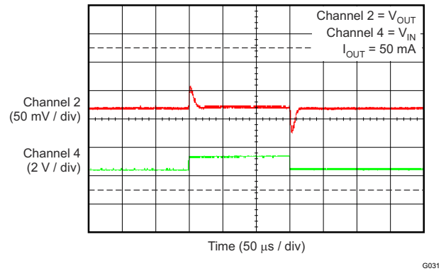
图 6-32. TPS70933 Line Transient (4.3 V to 5.3 V)
