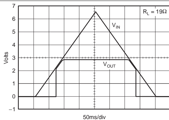
Figure 25. TPS799285 Power-Up/Power-Down
