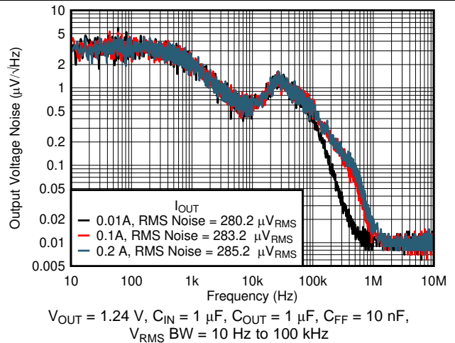
Figure 16. Output Noise ( V_n ) vs Frequency and I_{OUT}
