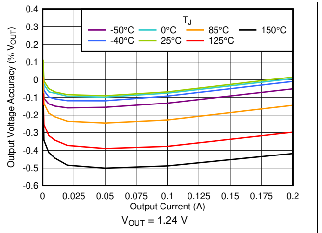
Figure 2. Load Regulation vs I_{OUT}
