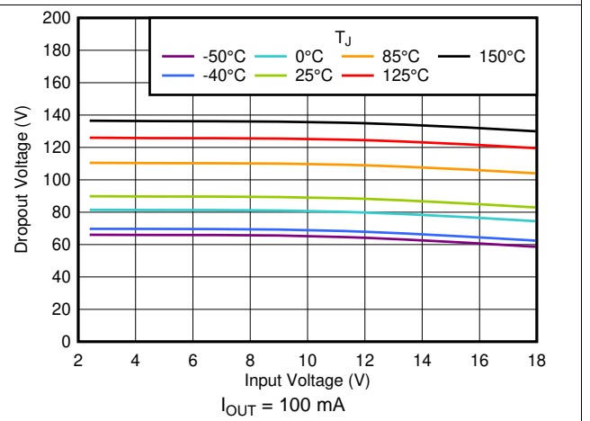
Figure 4. Dropout Voltage vs V_{IN}
