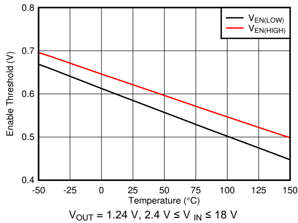
Figure 13. V_{EN} vs Temperature
