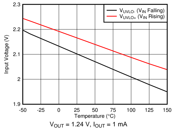
Figure 14. UVLO Thresholds vs Temperature
