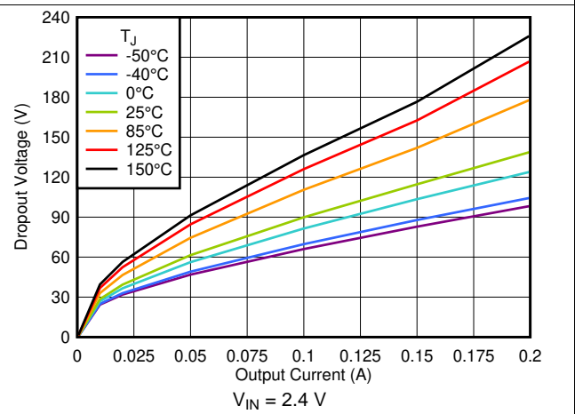
Figure 6. Dropout Voltage vs I_{OUT}
