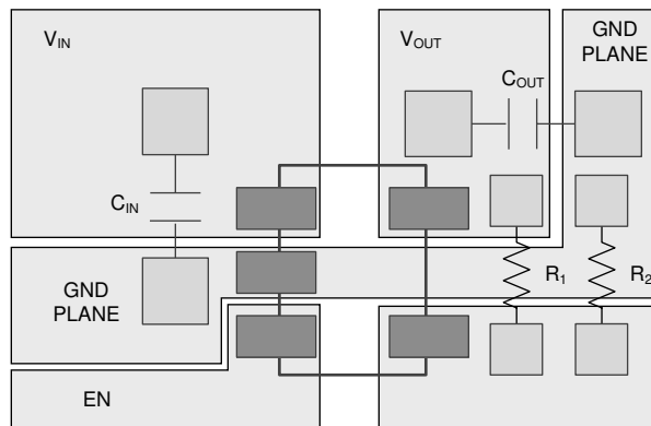
Figure 25. Adjustable Version Layout Example
