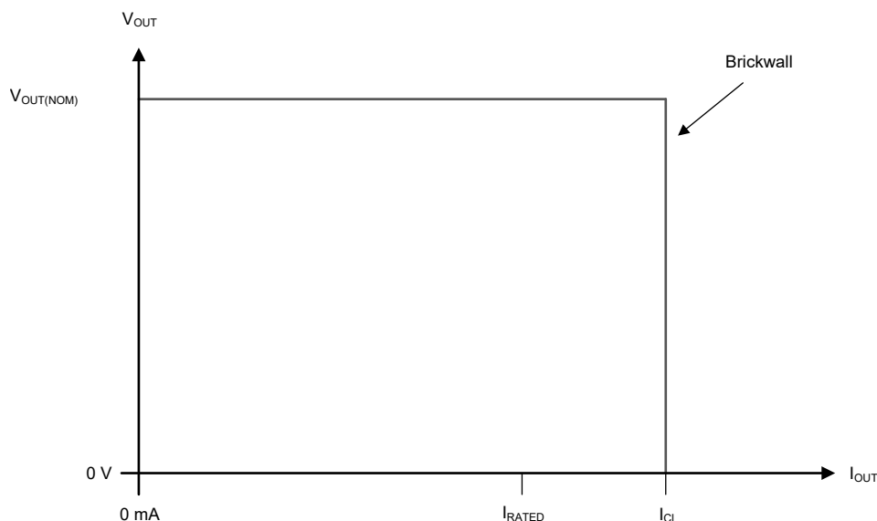
Figure 19. Current Limit
