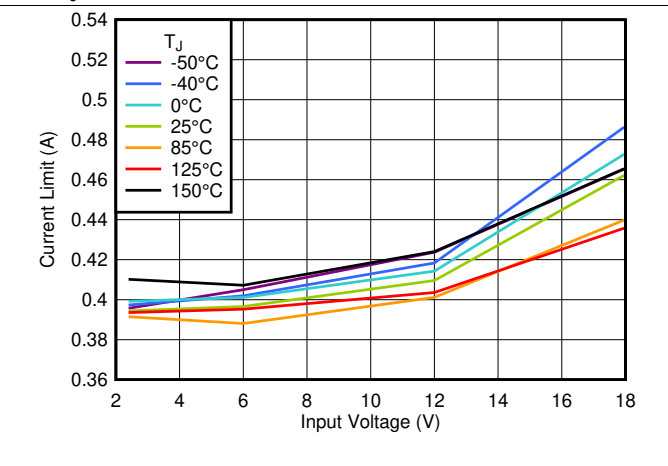
Figure 8. Current Limit vs V_{IN}
