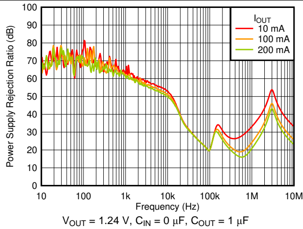
Figure 15. PSRR vs Frequency and I_{OUT}
