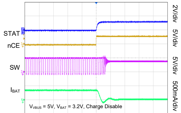
Time (5μs/div)
