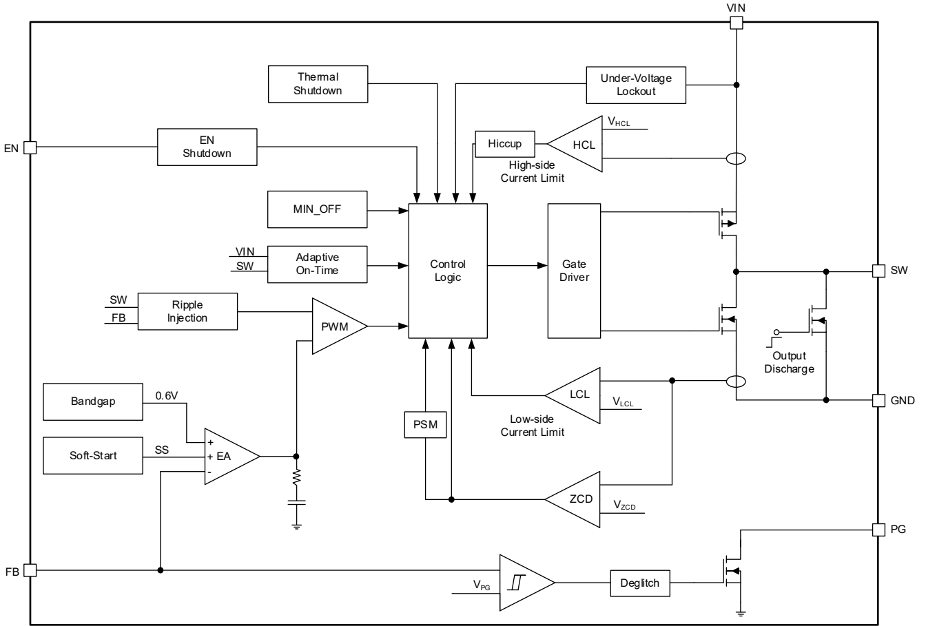
Figure 2. Block Diagram
