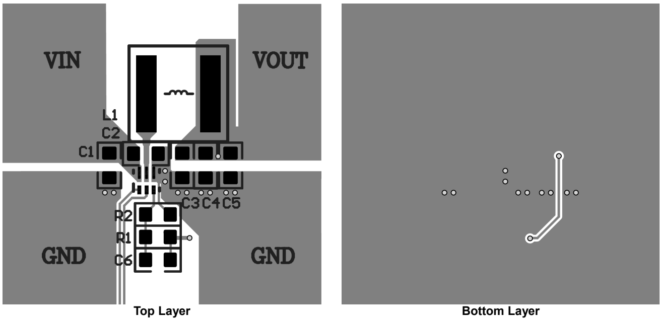
Figure 4. PCB Layout
