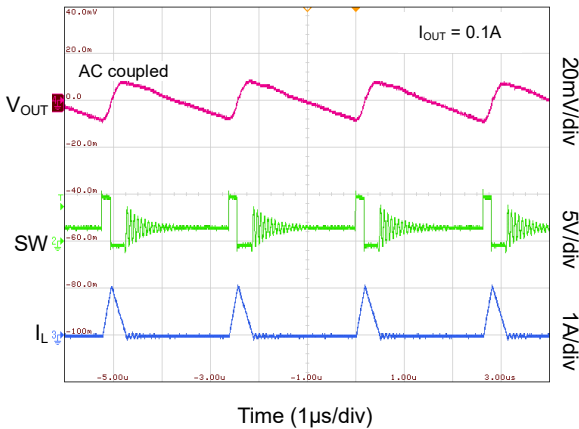
PSM Operation (SGM61024A)
