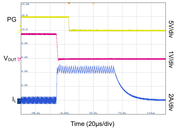
Hiccup Zoom In (SGM61024B)
