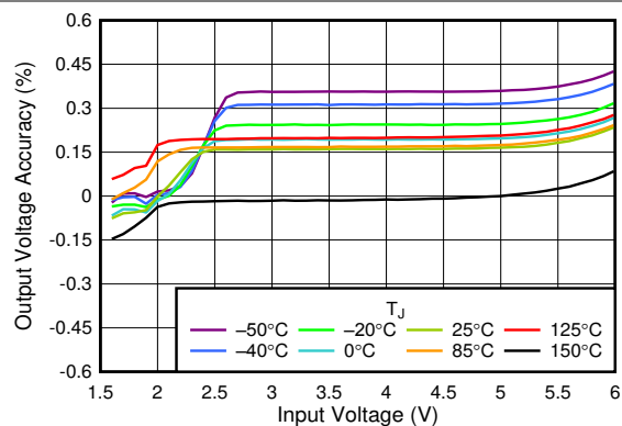
Figure 5-2. 0.55-V Line Regulation vs V_{IN}
