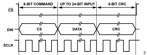
Figure 122. SPI Write Transaction with CRC
