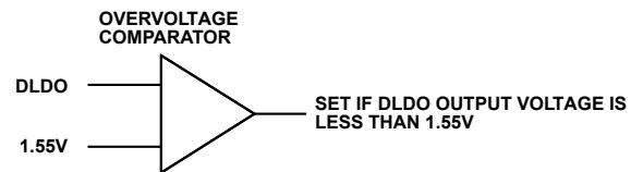
Figure 121. Digital LDO Monitor
