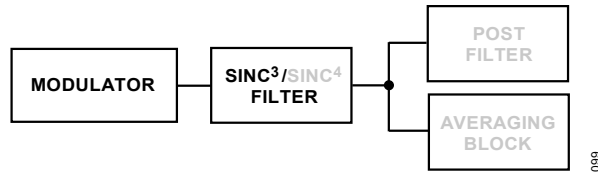
Figure 89. Sinc 3 Filter
