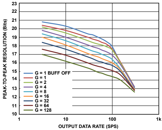
Figure 59. Peak-to-Peak Resolution vs. Output Data Rate, Sinc^3 + Sinc^1 Filter (Low Power Mode)
