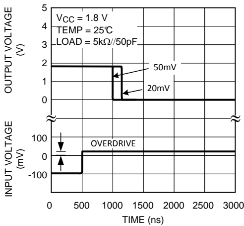
Figure 17. Propagation Delay (t PLH )
