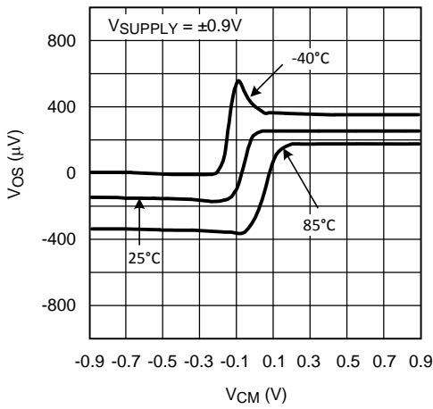
Figure 1. V OS vs. V CM
